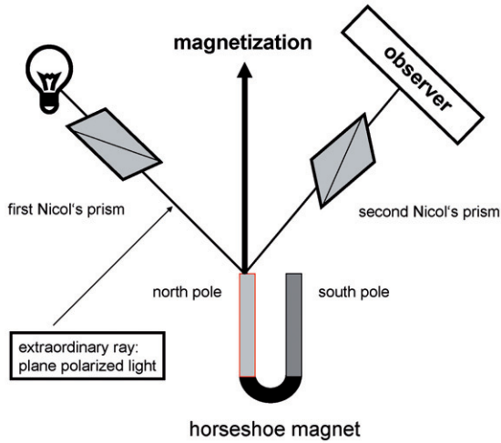
Figure 1. Experimental set-up used by John Kerr as described in [1]. According to his descriptions, the angle between the incident beam and the surface normal (magnetization) is between 60 and 80^\circ .
